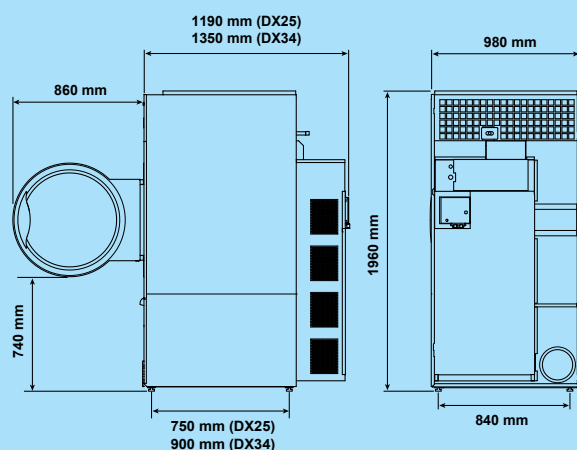
Side DX 34
